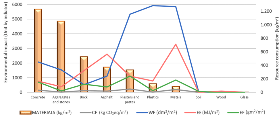
Fig. 10. Results per family of materials during the construction stage.
