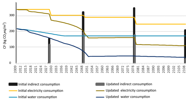
Fig. 11. Comparison of the evolution of CF in the BLC, before and after the environmental updates of the energy mix. Average proportion of the projects analysed.
